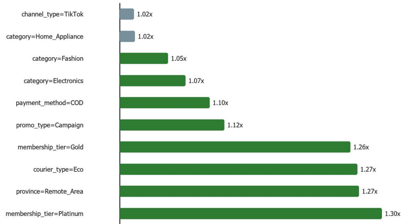
Graph 01: Categorical Impact
